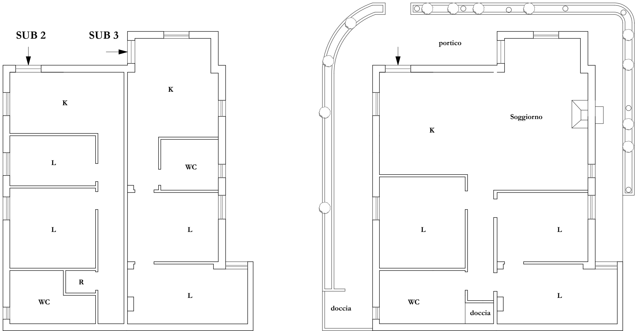
Fig. 6 part. 410 - Piano Seminterrato
